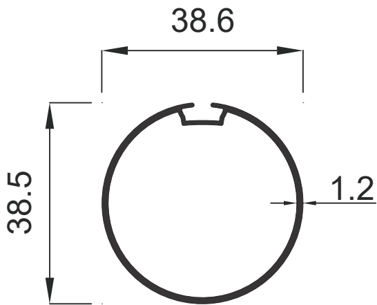
1221 0.393 Kg / m
