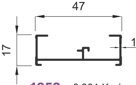
1958 0.301 Kg / m
