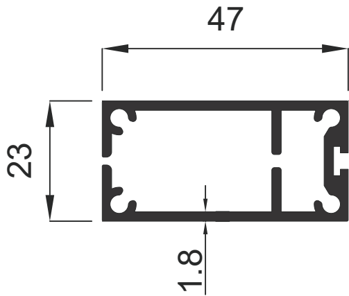
2573 0.827 Kg / m
