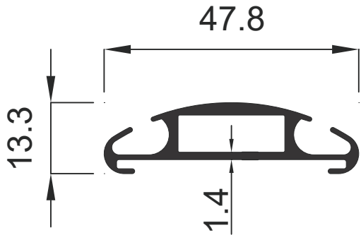
2532 0.440 Kg / m
